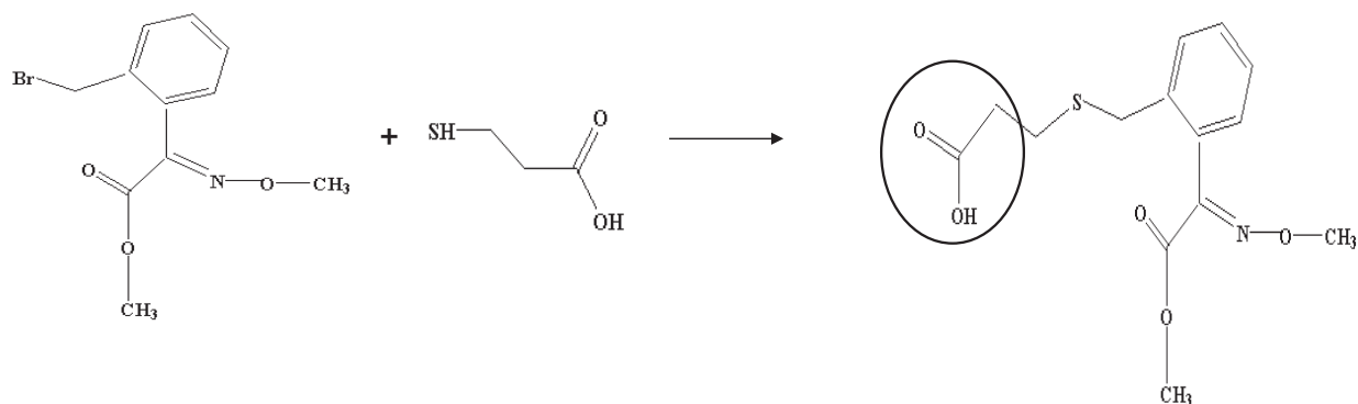
Figure 1. The synthesis of hapten. The OEBR reacted with mercaptopropionic acid to introduce a carboxyl group (in the circle) and synthesise hapten
