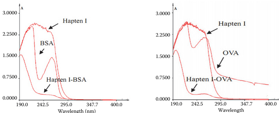
Figure 2. UV absorption spectrum of the hapten coupling with bovine serum albumin (BSA) or ovalbumin (OVA)
