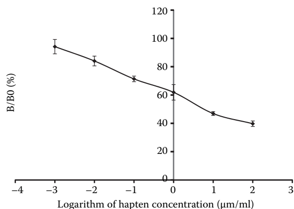
Figure 3. Standard curve for the indirect competitive hapten ELISA, y = -11.232x + 60.742 , R^2 = 0.9949
