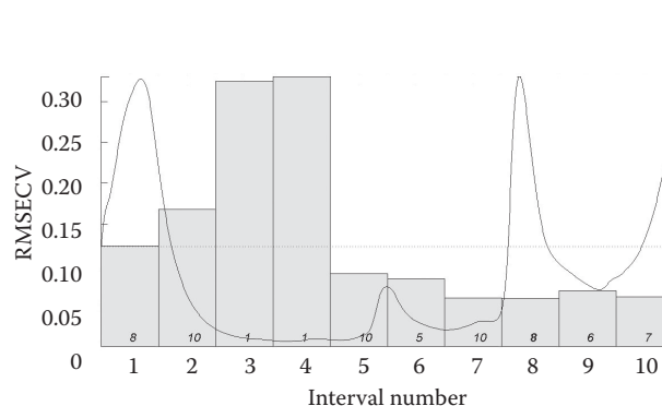
Figure 2. RMSECV of dark soy sauce's iPLS calibration model ( n = 10 )
