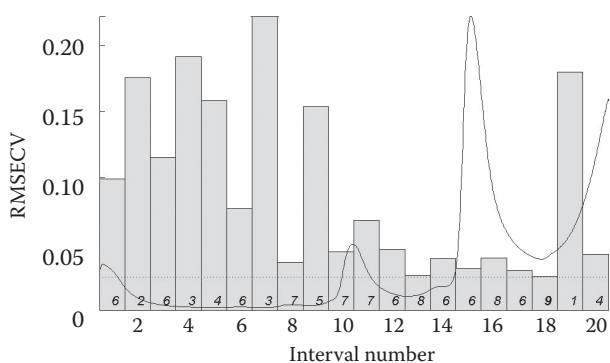
Figure 1. RMSECV of light soy sauce's iPLS calibration model ( n = 20 )
