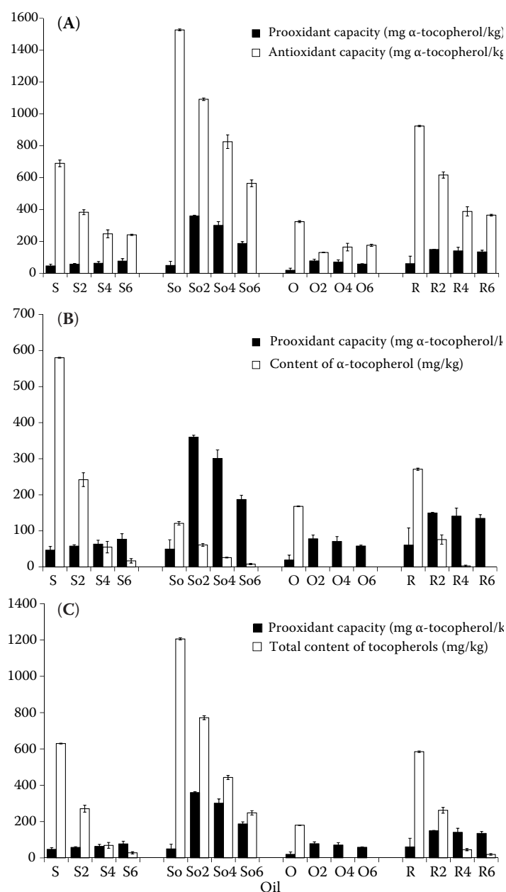
Figure 2. Comparison of prooxidant capacity with antioxidant capacity (A), content of \alpha -tocopherol (B), and total content of tocopherols (C) during heating of plant oils at temperature 180°C
