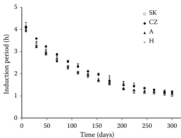
Figure 1. Oxidative stability of investigated sunflower oils expressed as induction periods determined by the Rancimat test under accelerated conditions (110°C, 20 l/h air flow)
