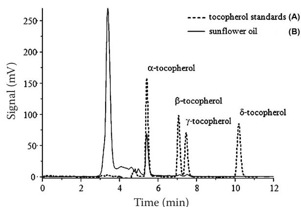
Figure 2. Determination of individual tocopherols by HPLC: (A) chromatogram of individual tocopherols determined in a model mixture composed of tocopherol standards and (B) chromatogram of individual tocopherols naturally present in the sample of initial sunflower oil (SK) used in the storage experiment
