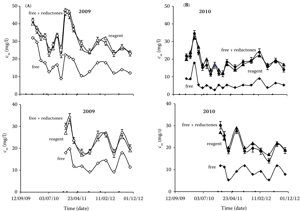
Figure 7. Comparison of free \text{SO}_2 content determined by the FSC method, free \text{SO}_2 content determined with a standard commercially available agent (CSR), and total content of free sulphur dioxide and reductones determined by the FSC and RC methods: (A) Pinot Blanc, and (B) blue Frankish in 2009 and 2010
