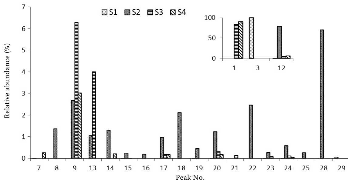
Figure 2. The impact of filtration on VOC identified in the samples of spirit S1–S4; analysed by HS-SPME/GC-MS. The numbers in the figure (Peak No.) correspond to the compounds listed in Tables 2 and 4
