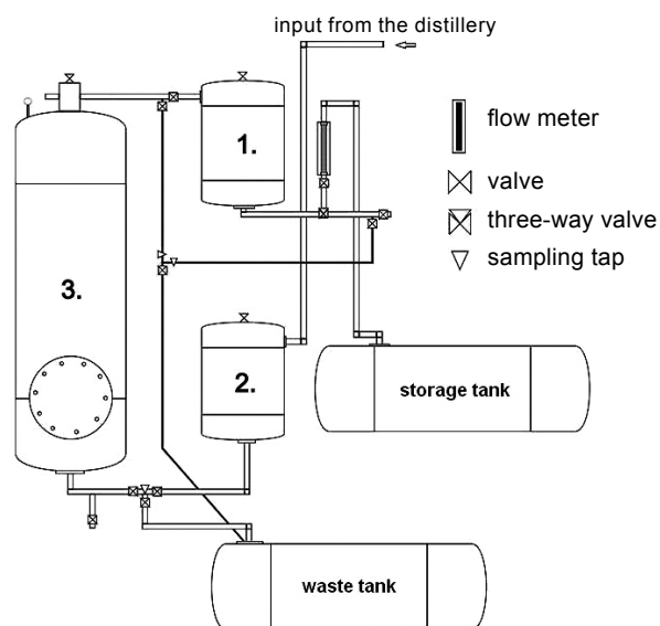
1 – first sand filter; 2 – second sand filter; 3 – filtration charcoal column
