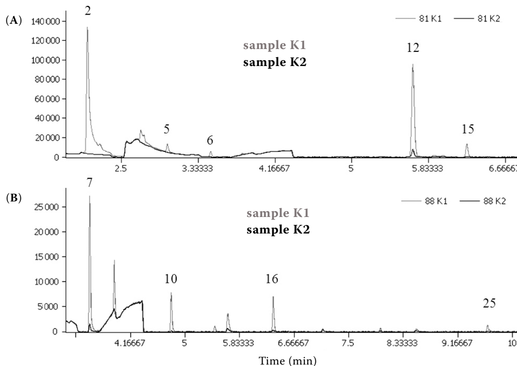
Figure 3. Chromatograms of Czech vodka samples K1 and K2: (A) a record of the characteristic ion ( m/z 88) of ethyl esters of carboxylic acids, (B) a record of the ion ( m/z 81) of substituted furans; the peak numbers in the chromatograms correspond to the compounds listed in Table 4
