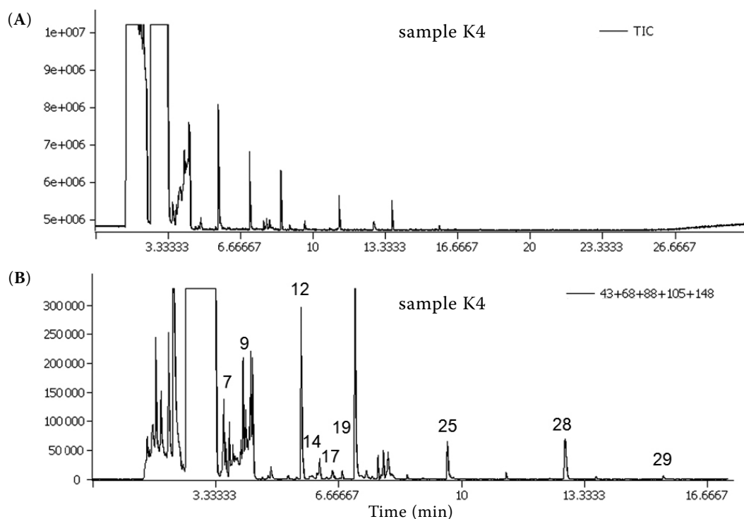
Figure 4. Chromatogram of Russian vodka K4: (A) Total Ion Current (TIC), (B) a record of selected m/z 43, 68, 88, 105, 148; the peak numbers in the chromatogram correspond to the compounds listed in Table 4
