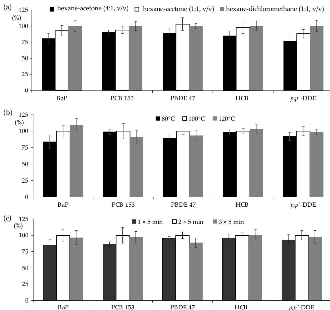
Figure 2. The effect of (a) extraction solvent mixture, (b) extraction temperature and (c) number of extraction cycles on the extraction efficiency of PLE for the most important representatives of PAHs, PCBs, PBDEs, and OCPs (BaP, PCB 153, PBDE 47, HCB, and p,p' -DDE). Optimised conditions shown in Figure 1. The results in the graphs represent mean values calculated from six replicates ( n = 6 )
