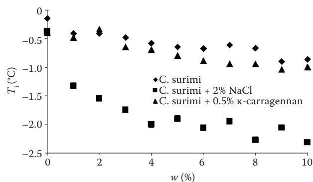
Figure 2. Initial freezing points ( T_i ) of chicken surimi as a function of mass fraction ( w ) of polydextrose and polydextrose in presence of 2% NaCl and 0.5% \kappa -carragennan
