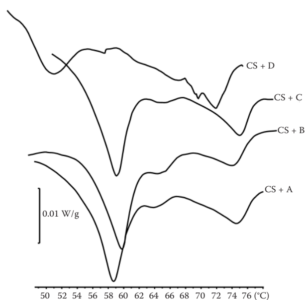
Figure 3. DSC thermograms of chicken surimi (CS) stored for 3 months at -25^{\circ}\text{C} mixed with: A (no additive), B (6% of polydextrose), C (0.5% of \kappa -carragennan and 6% of polydextrose), and D (2% NaCl and 6% of polydextrose)
