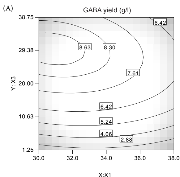
Figure 6. Contour plots (A) and response surface (B) for the effects on GABA yield of culture temperature (°C) ( X_1 ) and MSG addition (g/l) ( X_3 ) at initial pH 7.5
