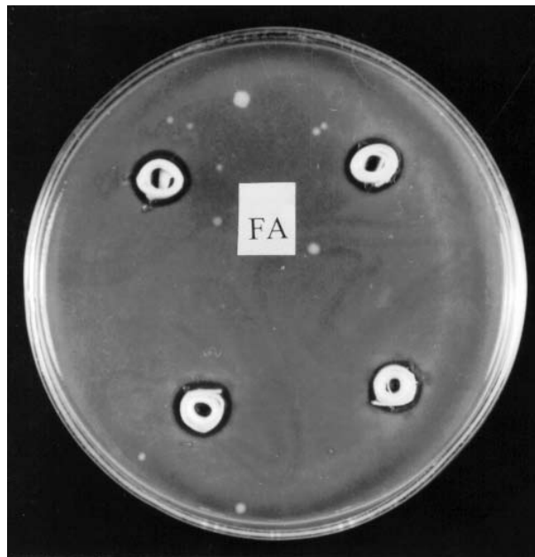
Figure 2. The formation of zones in plate with liquid malt agar by Bacillus subtilis around standard fusaric acid (FA) 200 mg/l.
