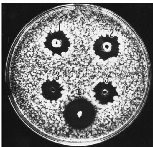
Figure 3. Transparent zones on plate with precultivated Bacillus subtilis by isolates of F. oxysporum (Schlecht) cultivated on solid malt medium. Isolates from (1) lentil seed, (2) lentil root, (3) isolate No. 545, and (3) isolate No. 485 and from (4) wheat cv. Agra
