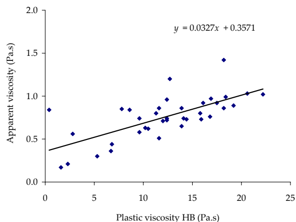
Figure 2. Relationship between the plastic viscosity (H-B) and the apparent viscosity
