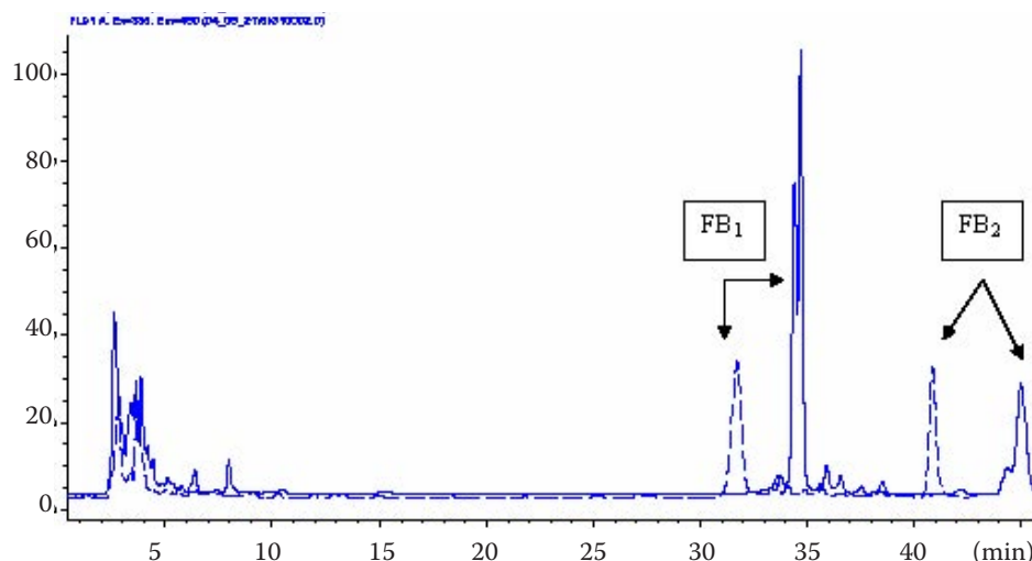
Figure 2. Chromatograms of split peaks at pH 2.9 (solid line) and non split peak at pH 2.6 (dashed line) in standard solution of FB 1 and FB 2
