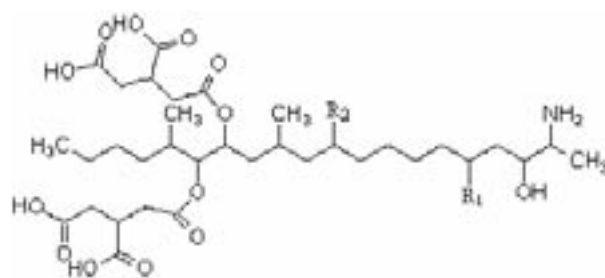
Figure 3. Chemical structure of FB 1 & FB 2
