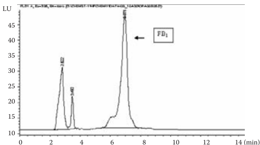
Figure 1. Chromatogram of isocratic separation with phosphate buffer at pH value 3.5. Fumonisin FB 1 standard
