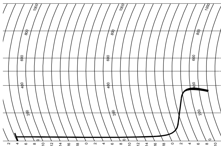
Figure 3. Amylogram of rice flour from MW treated sample (350 W, 100°C, moisture content 30%)
