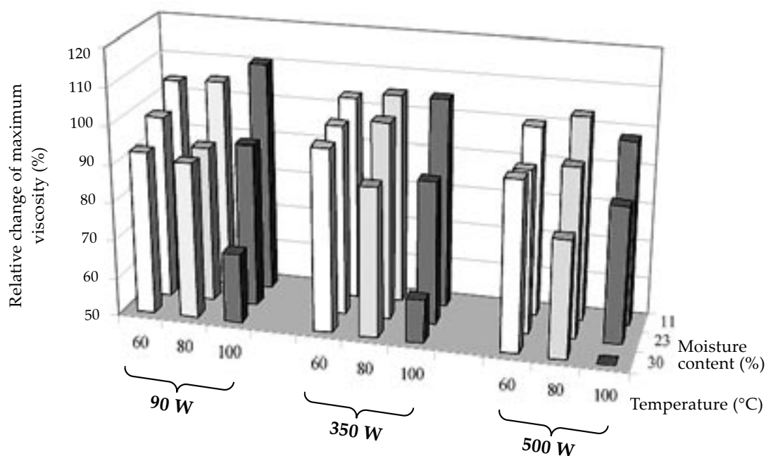
Figure 4. Evaluation of changes in maximum amylograph viscosity
