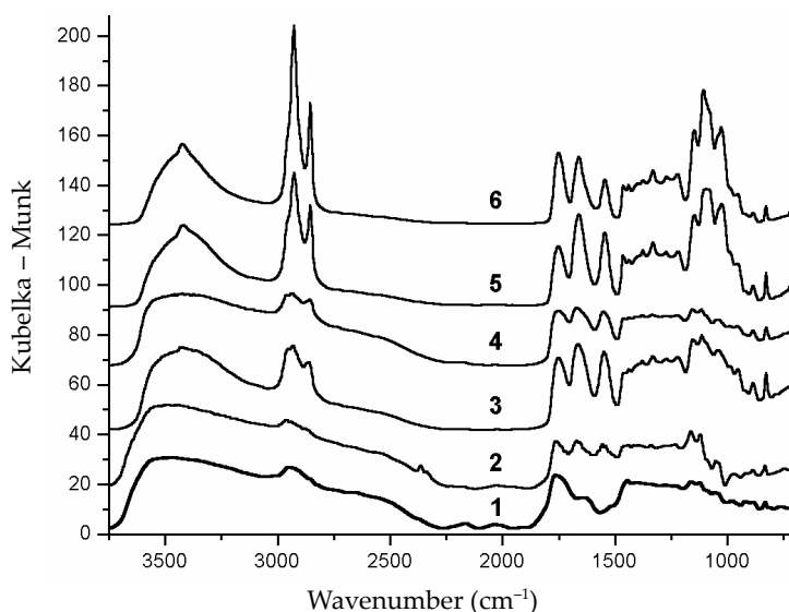
Figure 1. DRIFT spectra of HM citrus pectin 1 and N -alkylpectinamides 2–6
