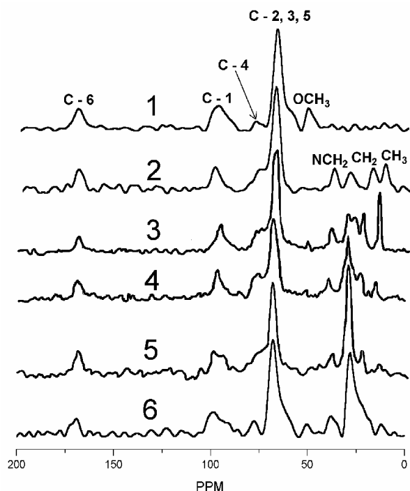
Figure 2. ^{13}\text{C} CP/MAS NMR spectra of HM citrus pectin 1 and N -alkylpectinamides 2–6
